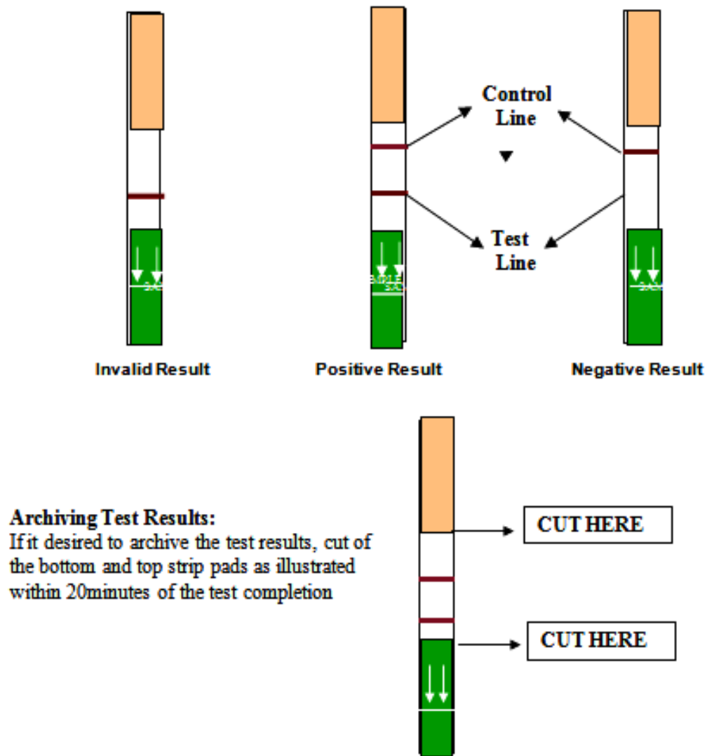
Figure 1: Schematic Representation of Lateral Flow Assay
