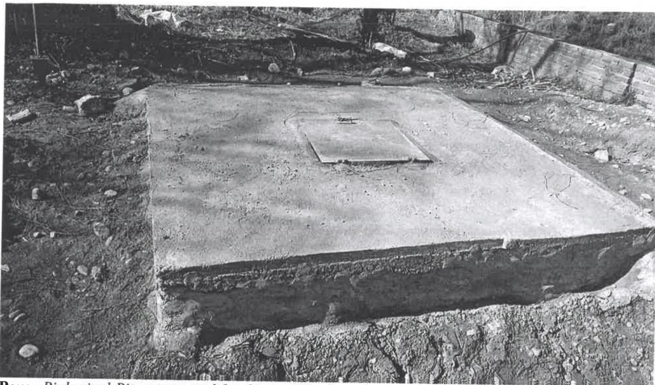
Paro: Biological Pit constructed for disposal food products, animal products and plant products
